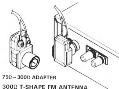
300Ω T-SHAPE FM ANTENNA
